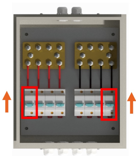
SET 8 XL: DC-4IN2OUT
