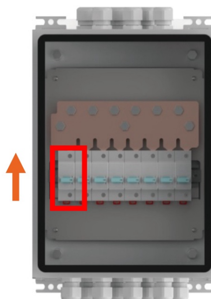
SET 12 XL & SET 16 XL: DC-8IN1OUT
